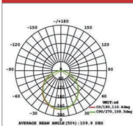
Luminus Intensity Distribution Diagram
