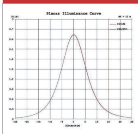
Planar Illuminance Curve
