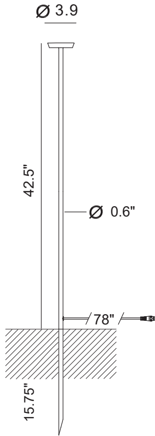
PIN MIDI - H3731-1080
