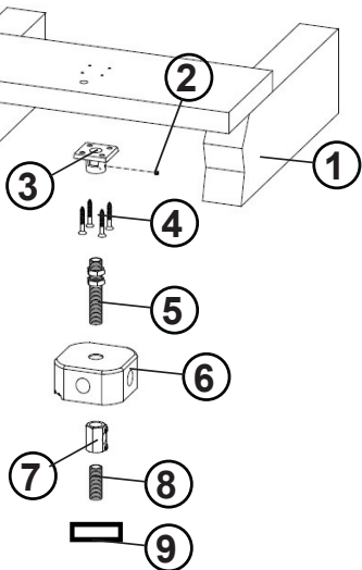
Drawing 2- Mounting over joist
