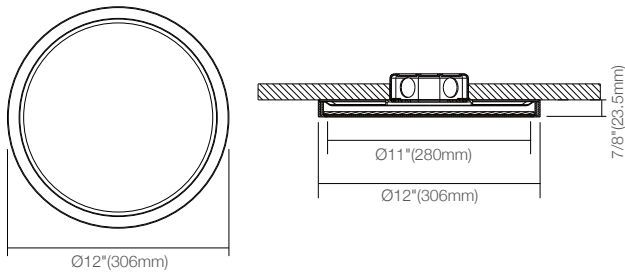
ADS12R-Tunable-5CCTYY (Plastic optional)
