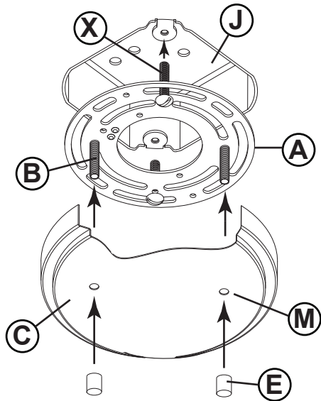
DRAWING 2 - MOUNTING
