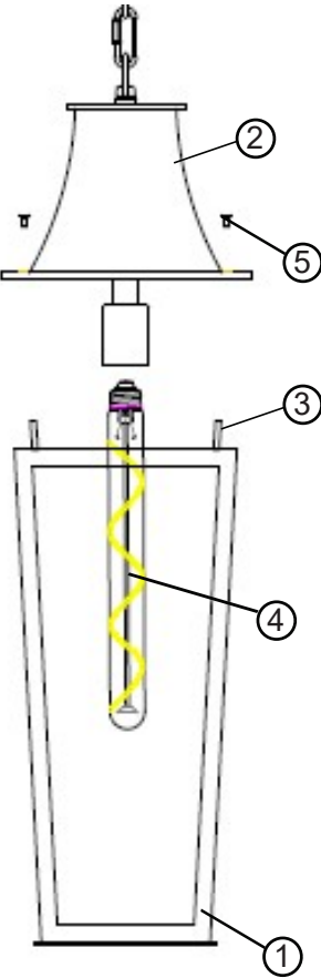
Drawing 2 - CAGE ASSEMBLY
