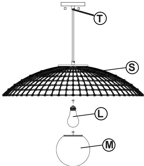
DRAWING 2- ASSEMBLY
