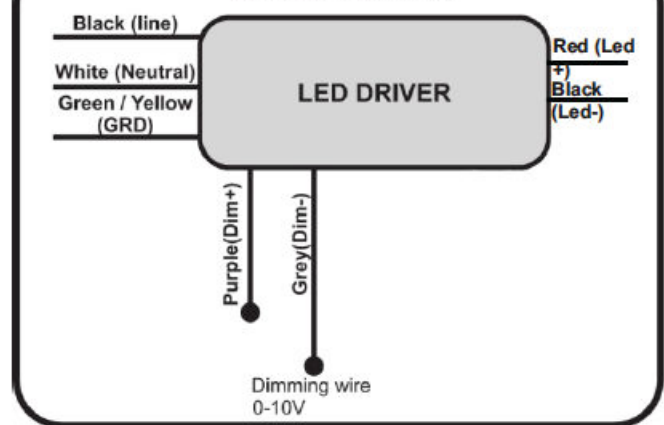
WIRING DIAGRAM
