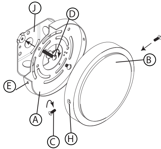
DRAWING 2- GLASS INSTALLATION
