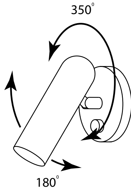
DRAWING 2 - ROTATION
