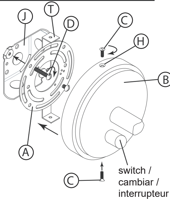
DRAWING 1 - MOUNTING
