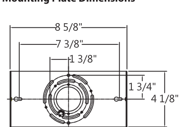
Mounting Plate Dimensions
