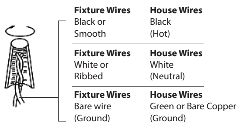
Fig.2 Wiring
