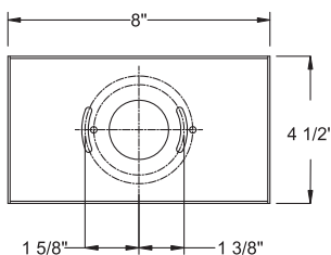
Conversion Plate Dimensions
