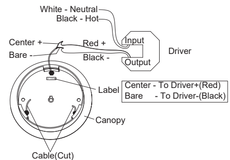
Fig.3 Driver Wires
