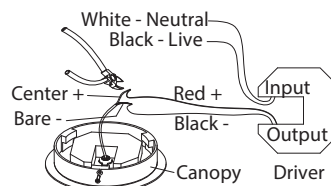
Fig.3 Driver Wiring
