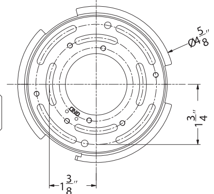
PD-30206 Back Plate Dimensions
