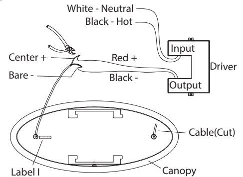
Fig.3 Driver Wires
