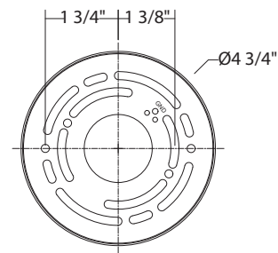
Mounting Back Plate
