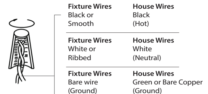
Fig.2 Wiring
