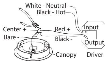
Fig.3 Driver Wiring
