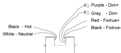
Fig. 3 Driver Wires
