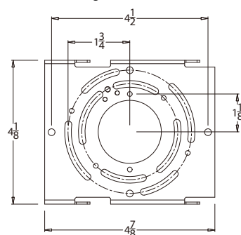
Mounting Plate Dimensions
