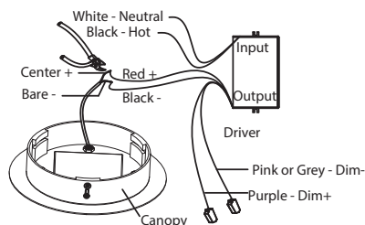
Fig.3 Driver Wires
