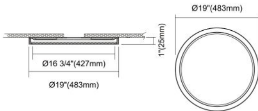
19" Die-cast Aluminum Round
